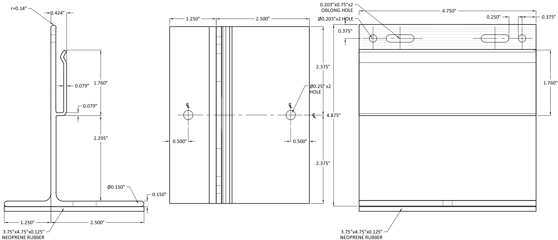
SIDE VIEW
